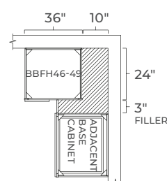
INSTALLATION DIAGRAM
