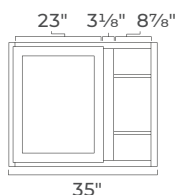
FACE FRAME OPENING DIMENSIONS
