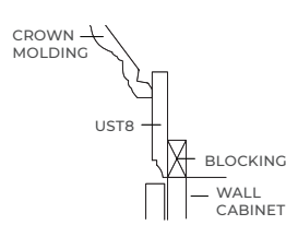
CROWN INSTALL DIAGRAM
