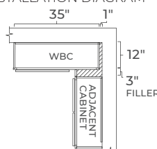
INSTALLATION DIAGRAM
