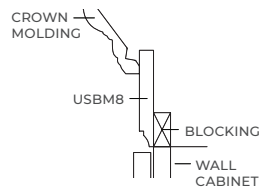
CROWN INSTALL DIAGRAM
