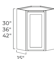
INSTALLATION DIAGRAM
