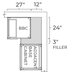
INSTALLATION DIAGRAM
