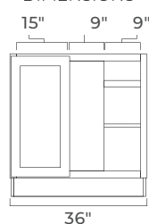
FACE FRAME OPENING DIMENSIONS
