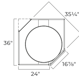
FACE FRAME OPENING DIMENSIONS
