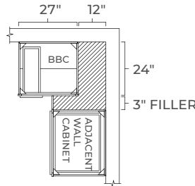
INSTALLATION DIAGRAM
