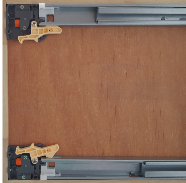
Full extension, undermount drawer glides with integrated soft close
